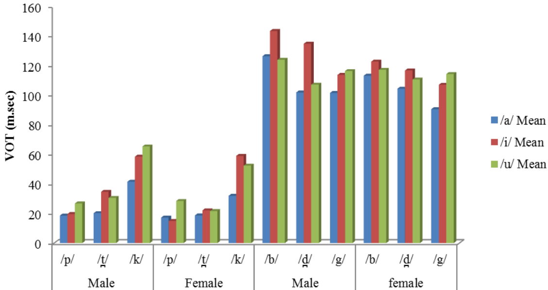
Figure 2. Shows the Mean VOT values for plosives across gender and across different vowel contexts
