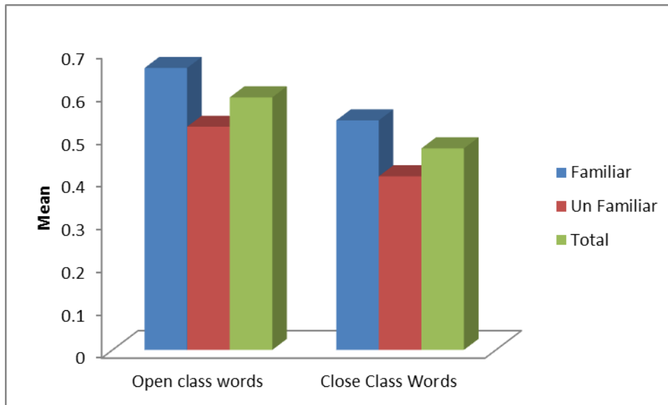
Figure (1) shows that there is a highly significant difference between open class and close class words for familiar and unfamiliar tasks.
